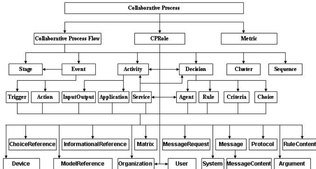
Figure 1: SOA Information Model (High Level)
